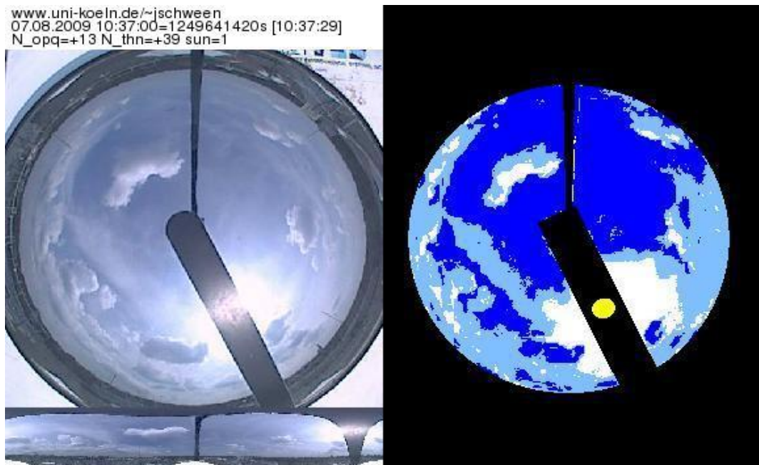
Figure 2: Exemplary sky image (left) together with cloud classification mask (right), time stamp, derived percentages of opaque and thin clouds and a flag indicating whether the sun is visible (top left). Colors in the cloud mask indicate sky (dark blue), thin clouds (light blue) and clouds (white). The yellow dot in the cloud mask at the sun position indicates that the sun is visible.
