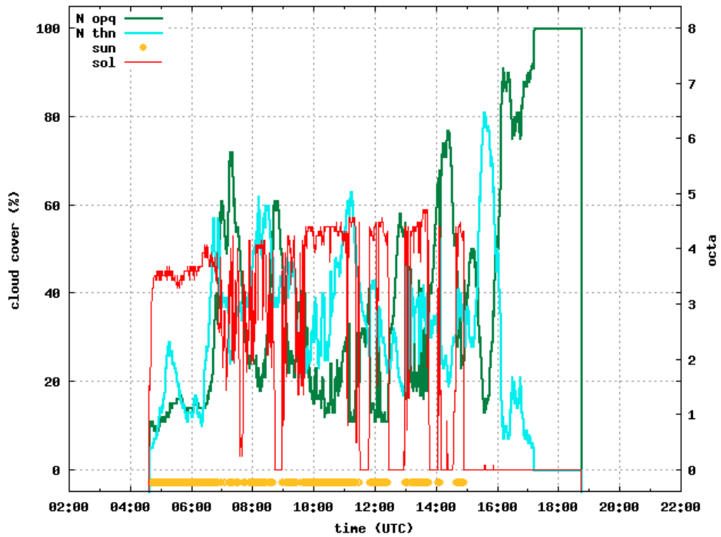
Figure 3: Exemplary quicklook from 7.8.2008 with N opq the percentage of opaque cloud pixels, N thn the percentage of thin cloud pixels and sol what the manufacturer calls 'solar strength'. Variable sun shows the sun visibility flag as an orange circle below the zero line when the sun is visible.
